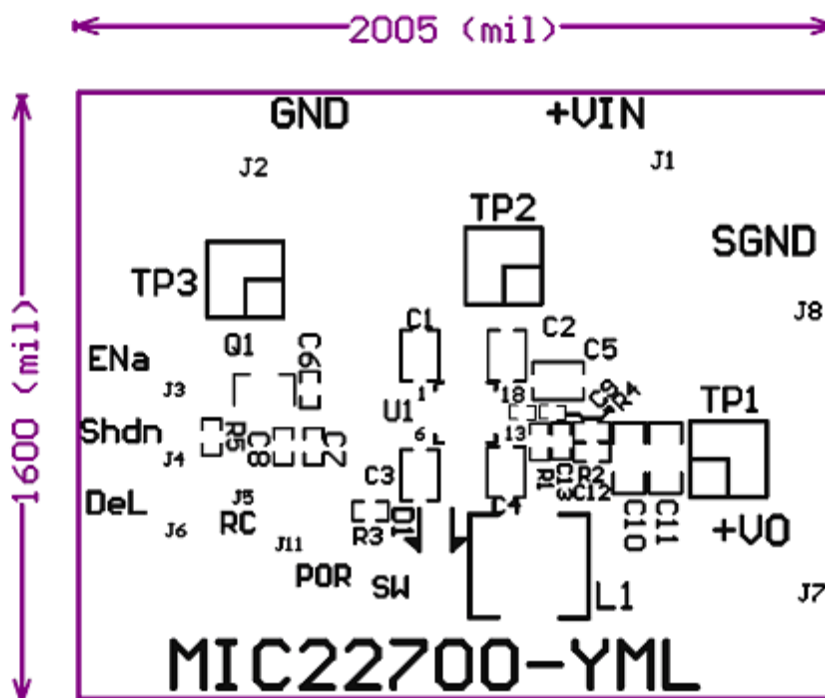
Top Silk
